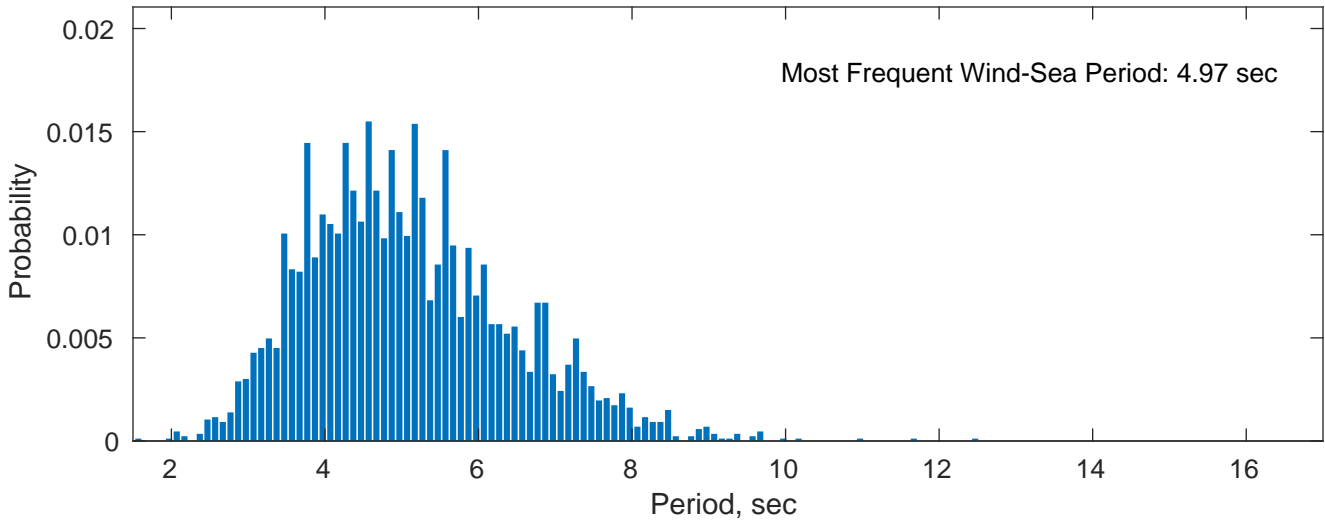
Wind-Sea: 40.09%
