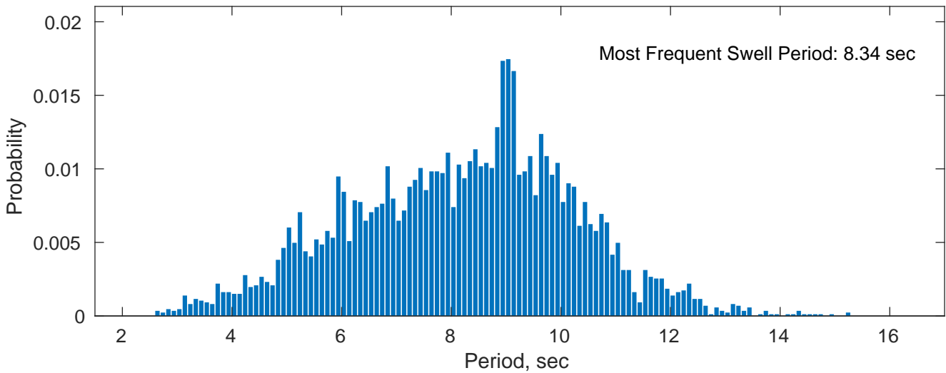
Swell: 59.91%
