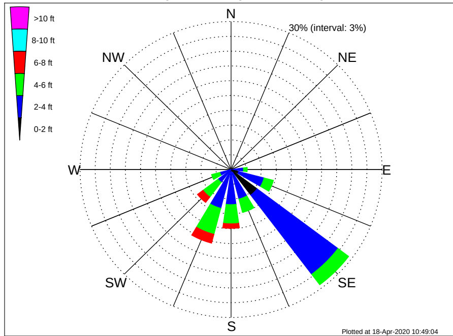
OCS A-0501 South Climatological WaveHeight Rose for August: 1979 - 2015
