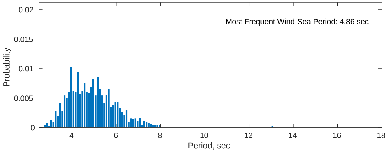
Wind-Sea: 19.22%
