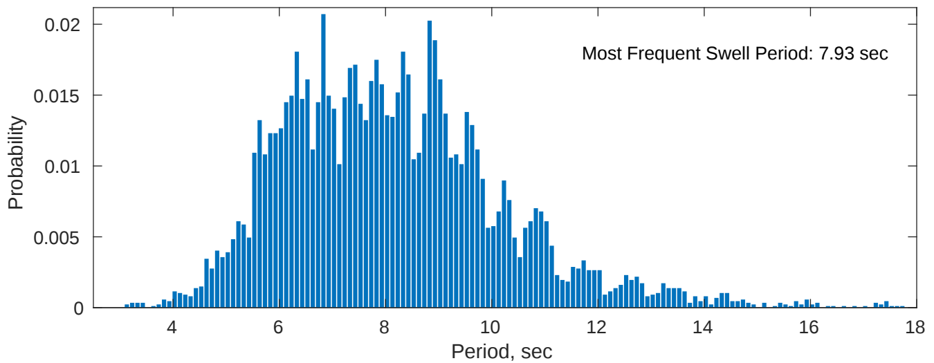
Swell: 80.78%
