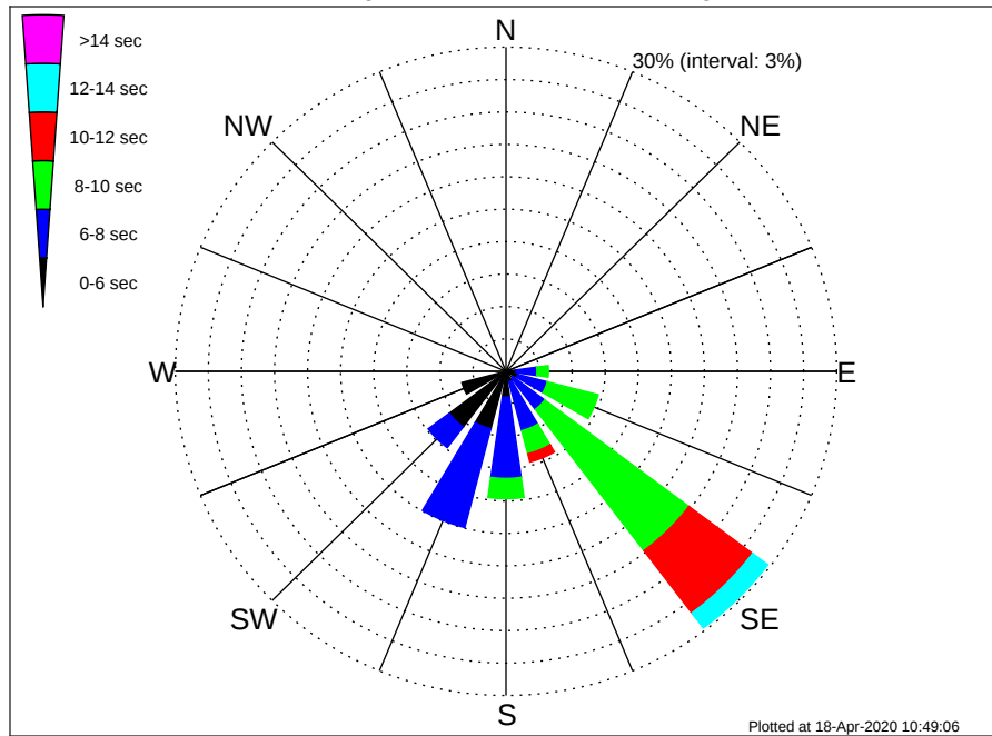
OCS A-0501 South Climatological WavePeriod Rose for August: 1979 - 2015
