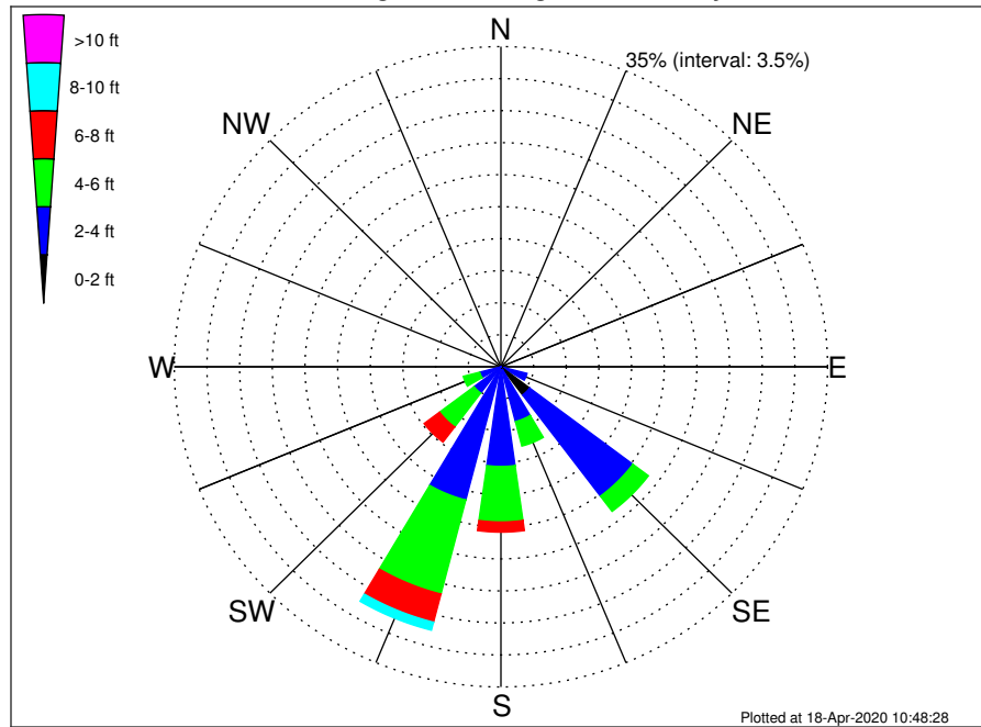
OCS A-0501 South Climatological WaveHeight Rose for July: 1979 - 2015
