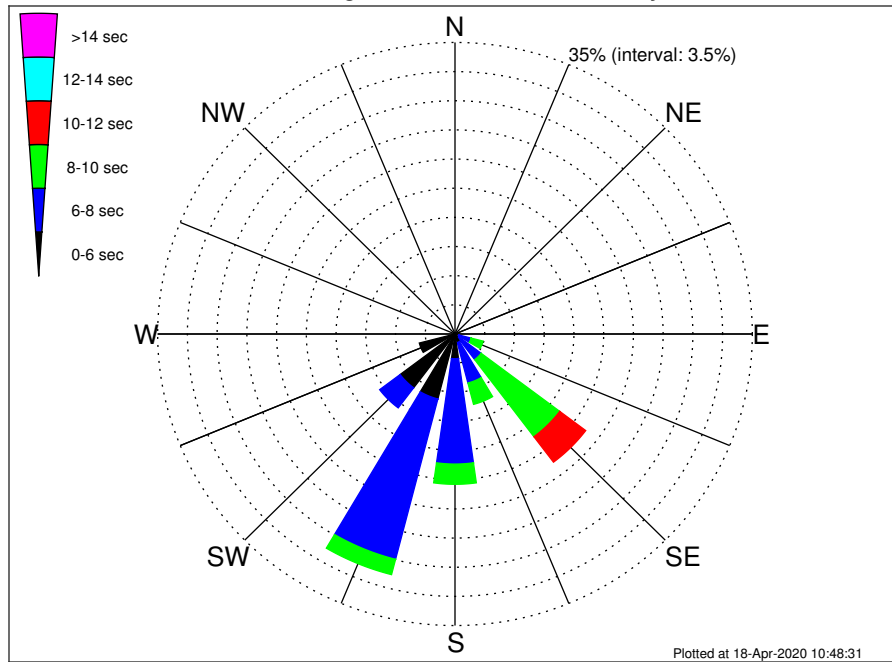
OCS A-0501 South Climatological WavePeriod Rose for July: 1979 - 2015
