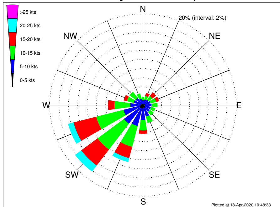
OCS A-0501 South Climatological Wind Rose for July: 1979 - 2015
