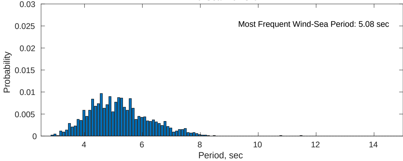
Wind-Sea: 20.18%
