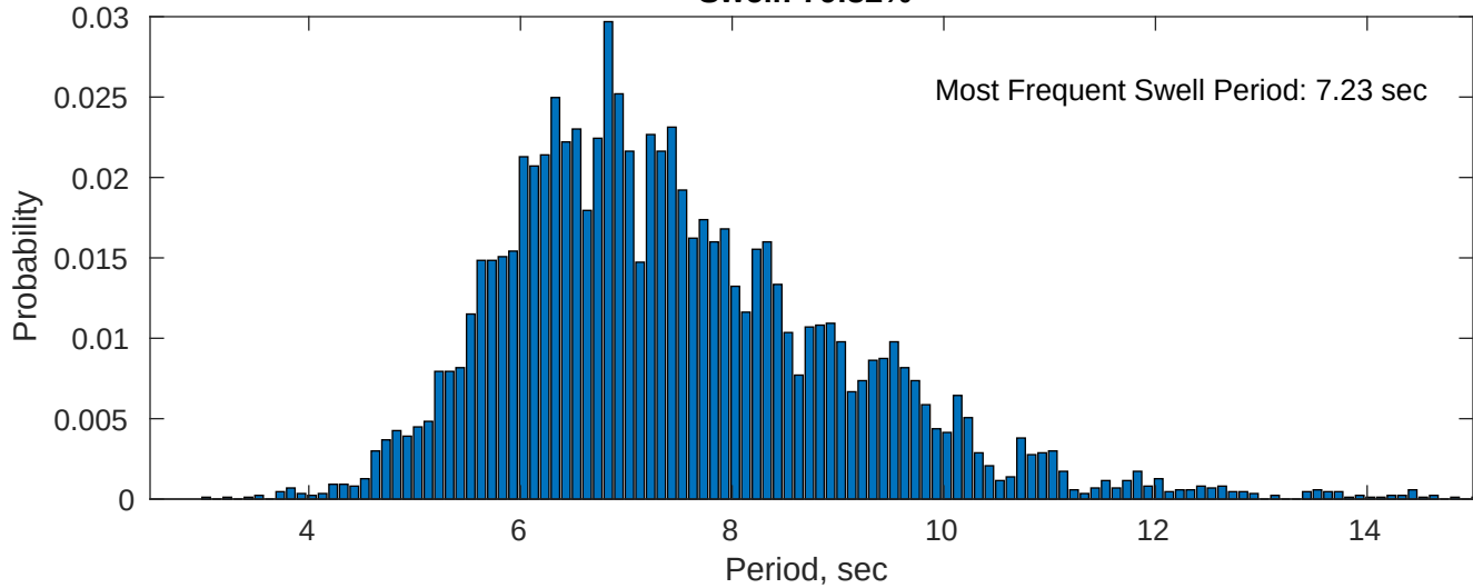
Swell: 79.82%
