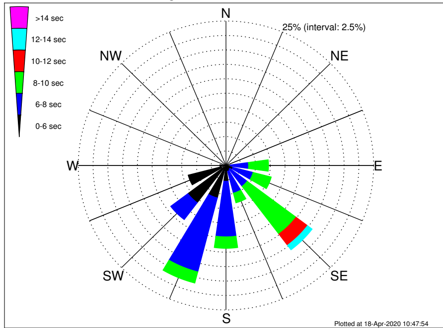
OCS A-0501 South Climatological WavePeriod Rose for June: 1979 - 2015
