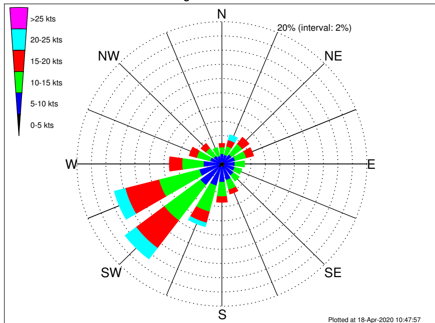
OCS A-0501 South Climatological Wind Rose for June: 1979 - 2015
