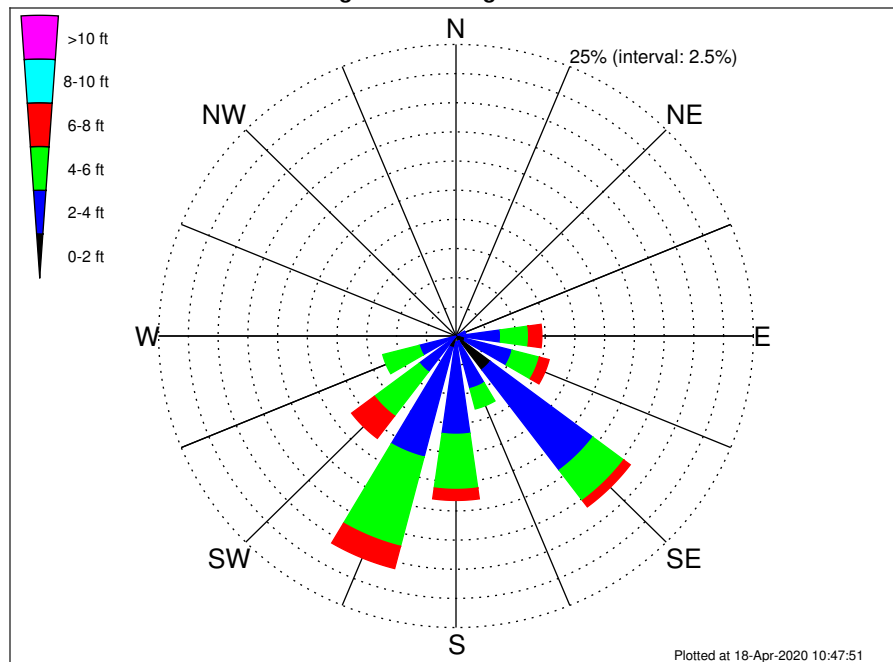
OCS A-0501 South Climatological WaveHeight Rose for June: 1979 - 2015
