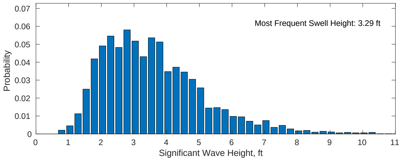
Swell: 76.17%
