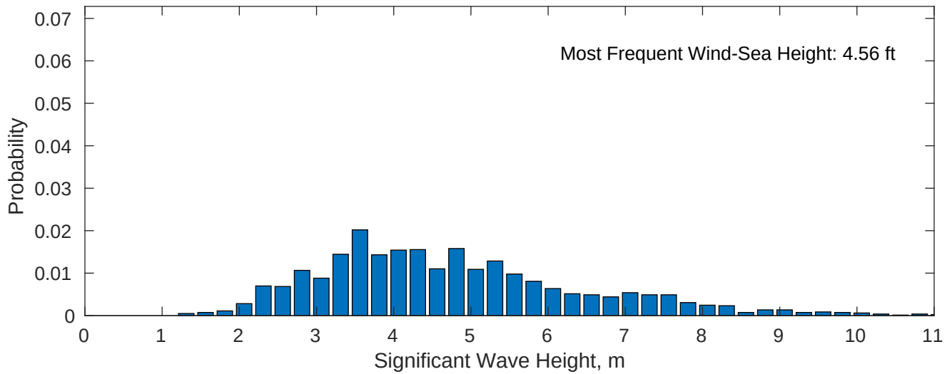
Wind-Sea: 23.83%
