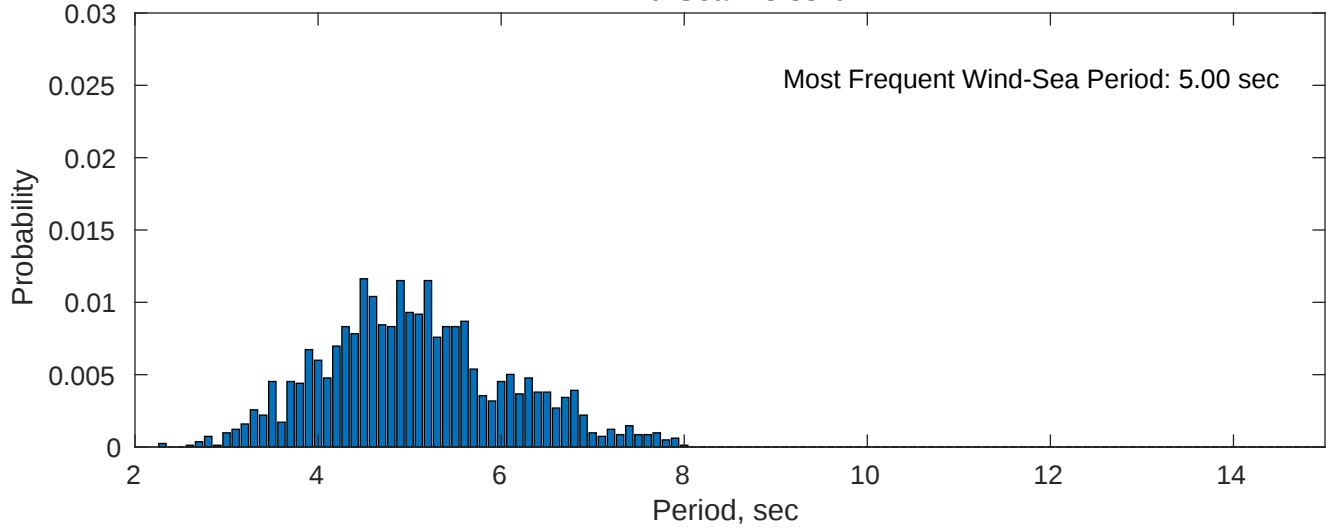
Wind-Sea: 23.83%
