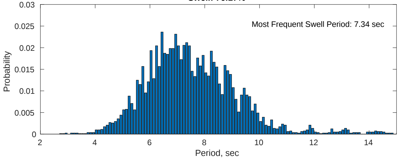
Swell: 76.17%
