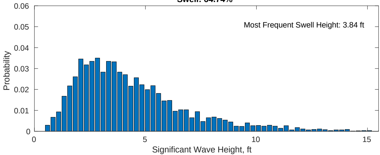
Swell: 64.74%
