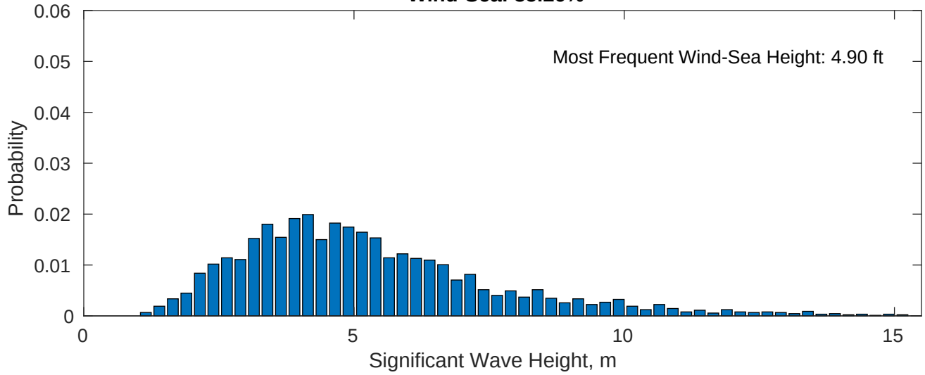
Wind-Sea: 35.26%
