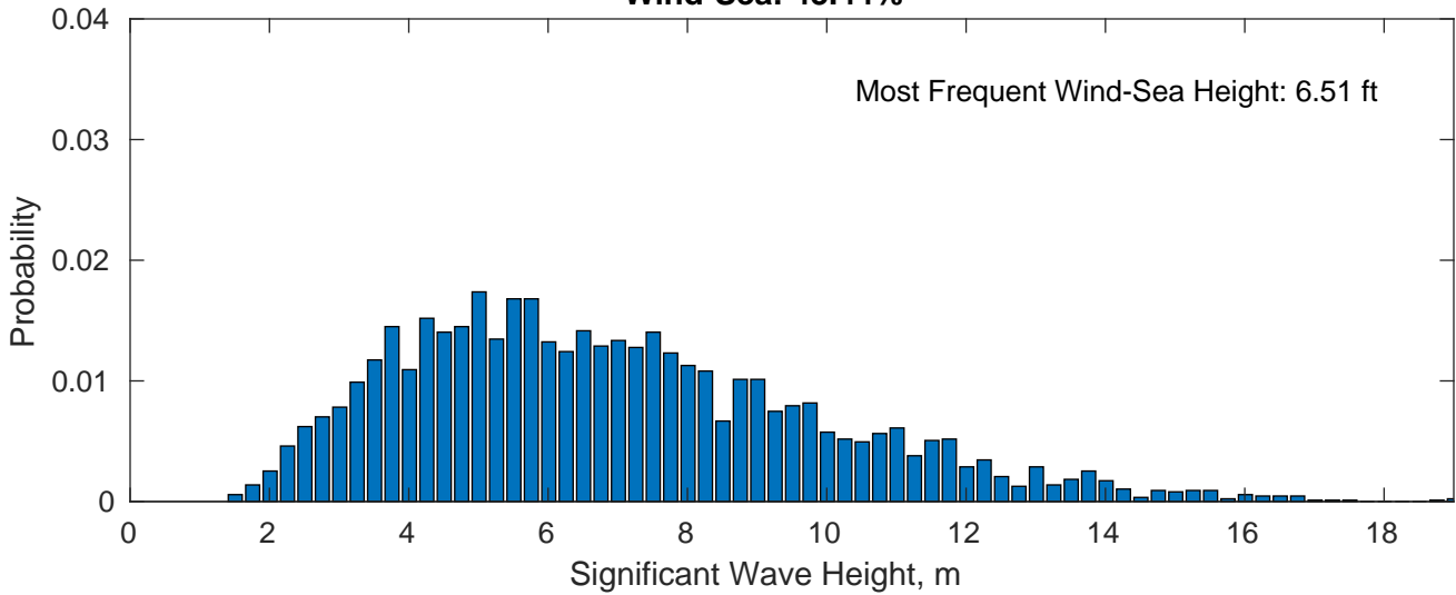
Wind-Sea: 43.44%
