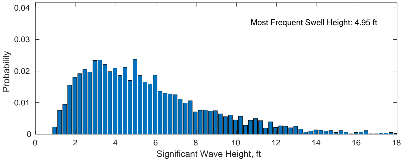
Swell: 57.01%
