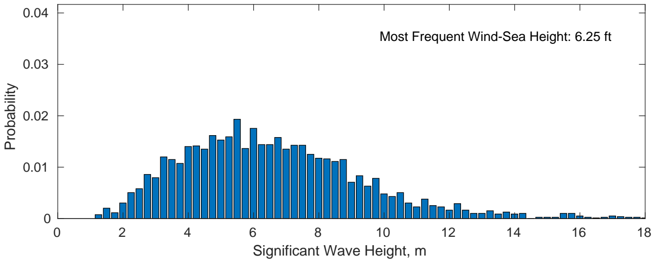
Wind-Sea: 42.99%
