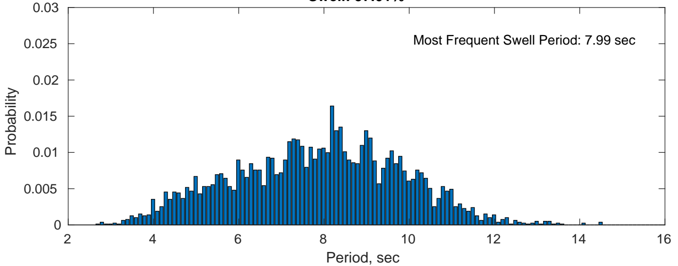
Swell: 57.01%
