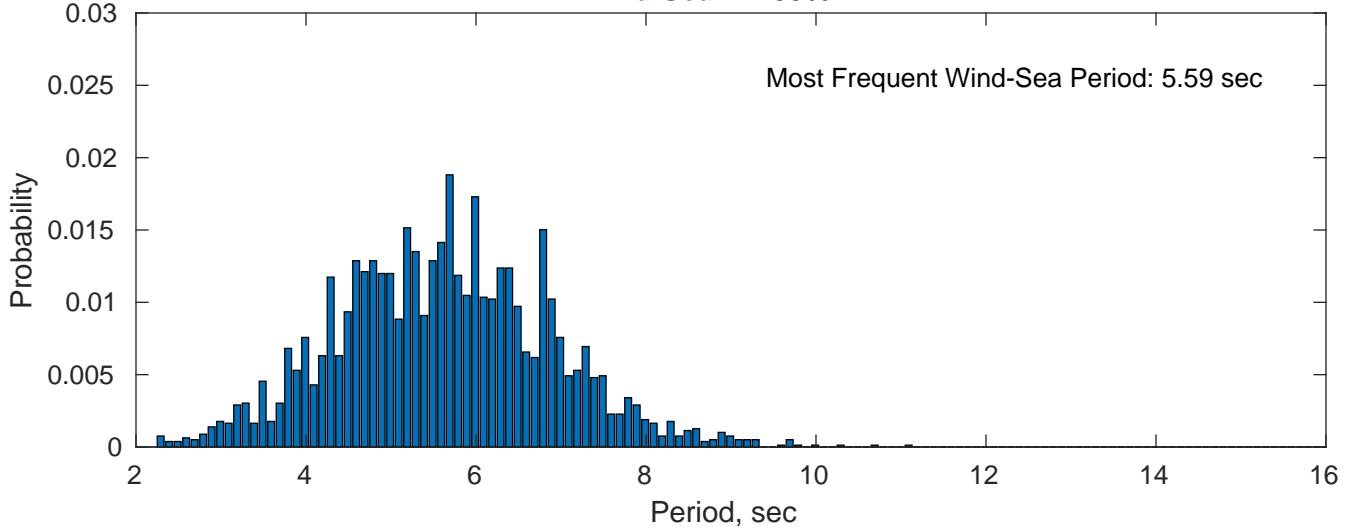
Wind-Sea: 42.99%
