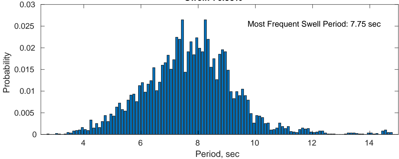
Swell: 76.38%
