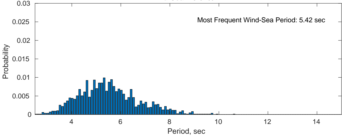
Wind-Sea: 23.62%
