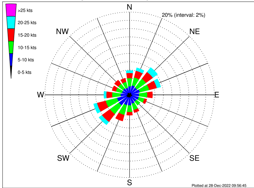
OCS A-0522 Climatological Wind Rose for September: 1979 - 2015
