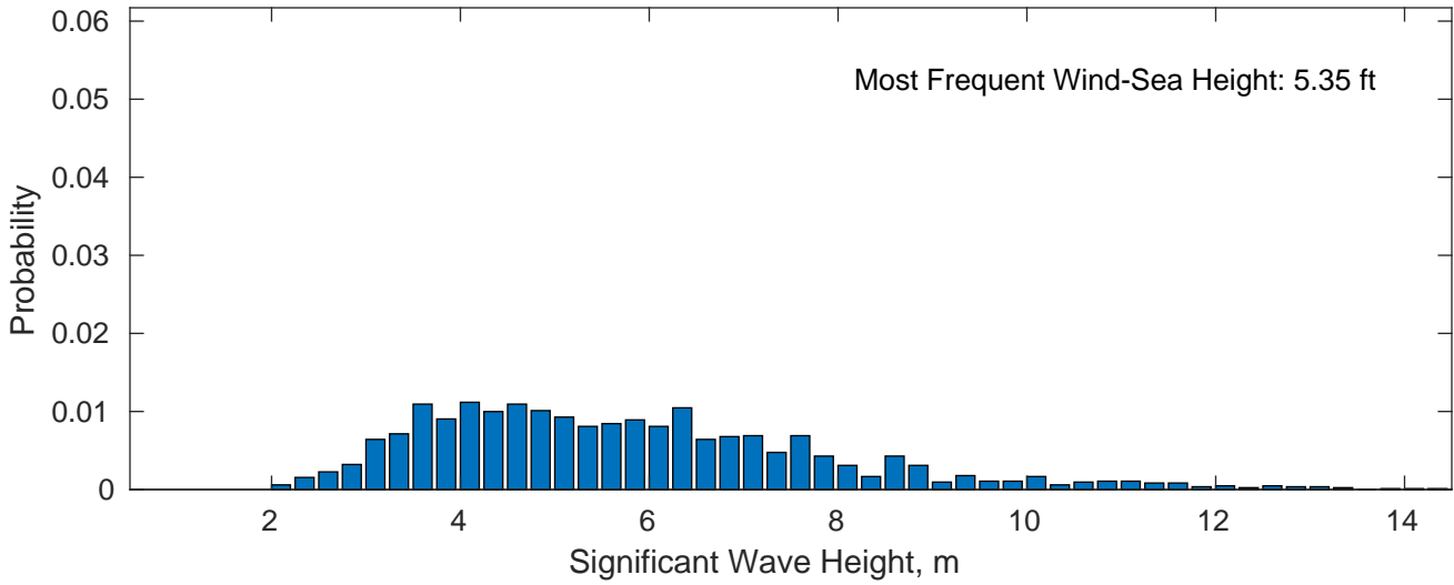
Wind-Sea: 20.13%
