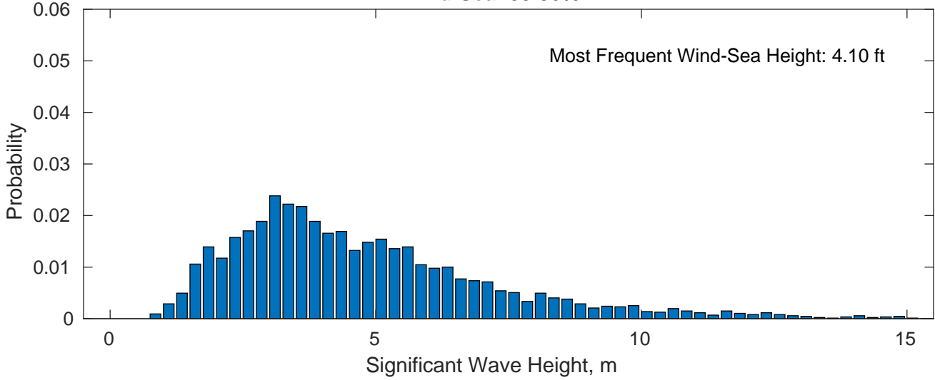
Wind-Sea: 39.86%
