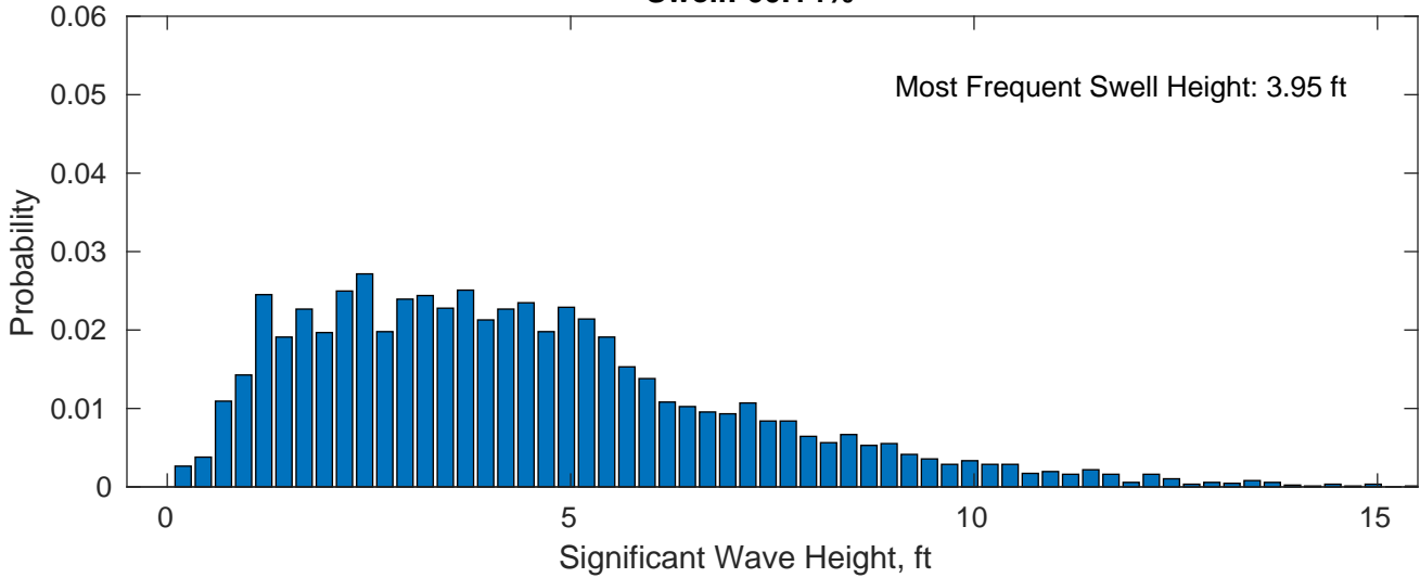
Swell: 60.14%
