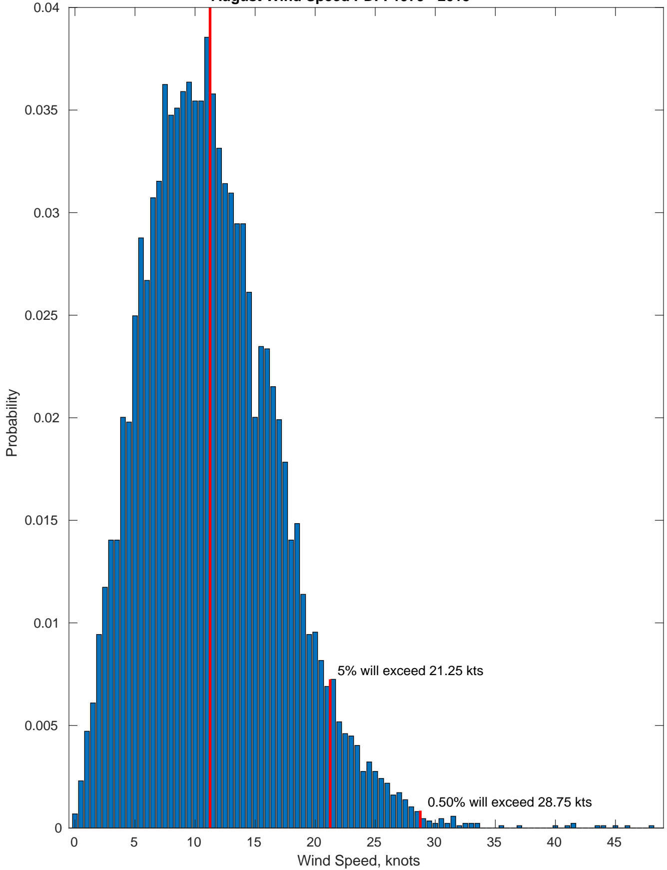
Most Frequent Wind Speed: 11.25 kts August Wind Speed PDF: 1979 - 2015
