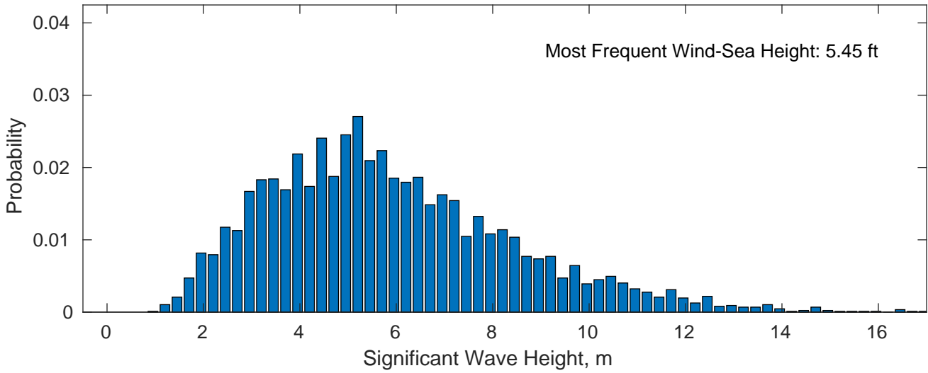
Wind-Sea: 52.83%
