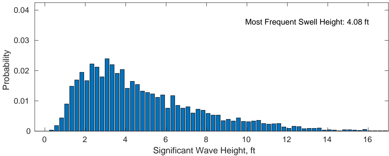
Swell: 47.17%
