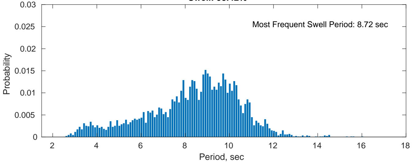
Swell: 58.42%
