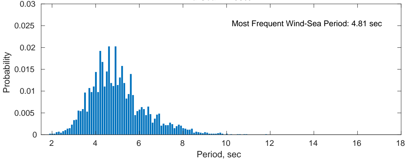
Wind-Sea: 41.58%
