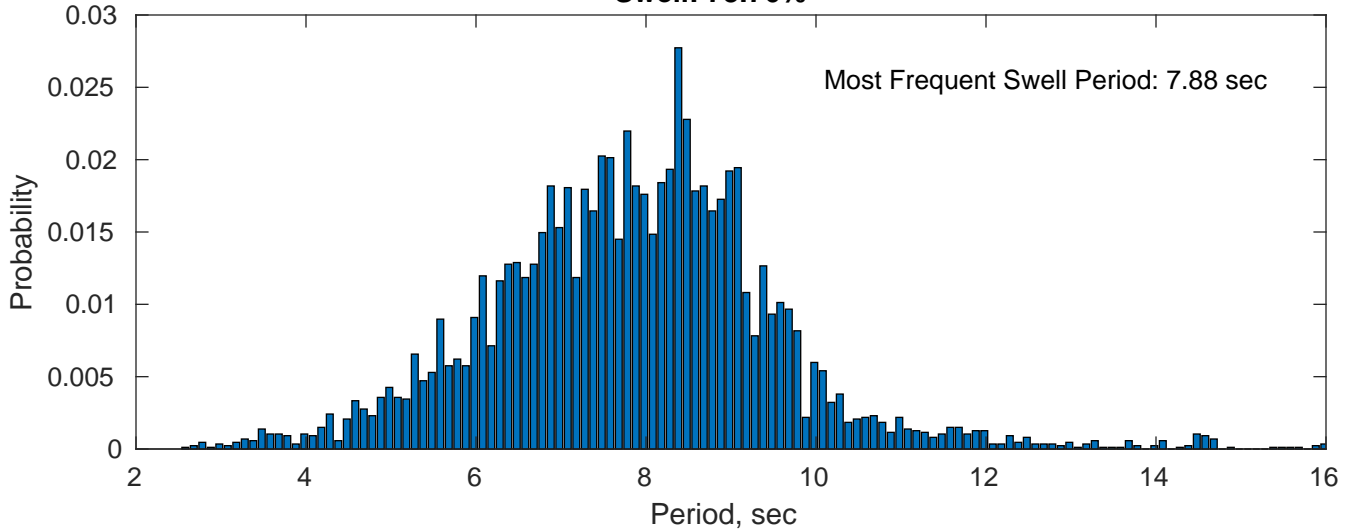
Swell: 73.76%
