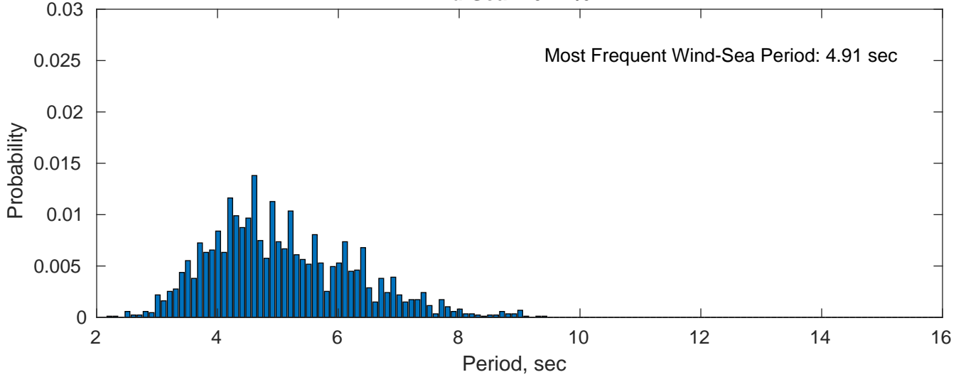
Wind-Sea: 26.24%
