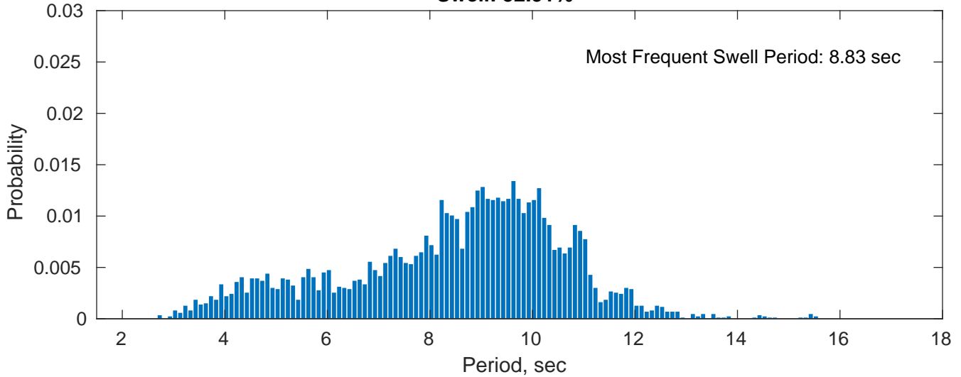
Swell: 52.91%
