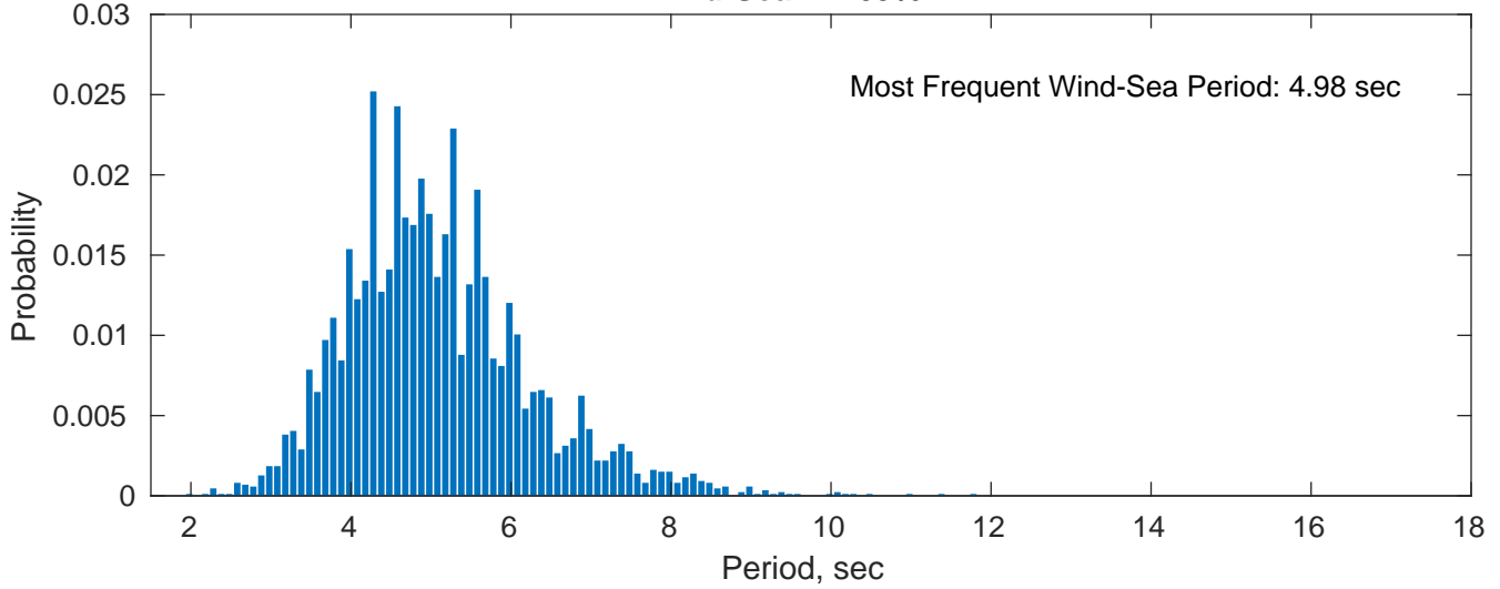
Wind-Sea: 47.09%
