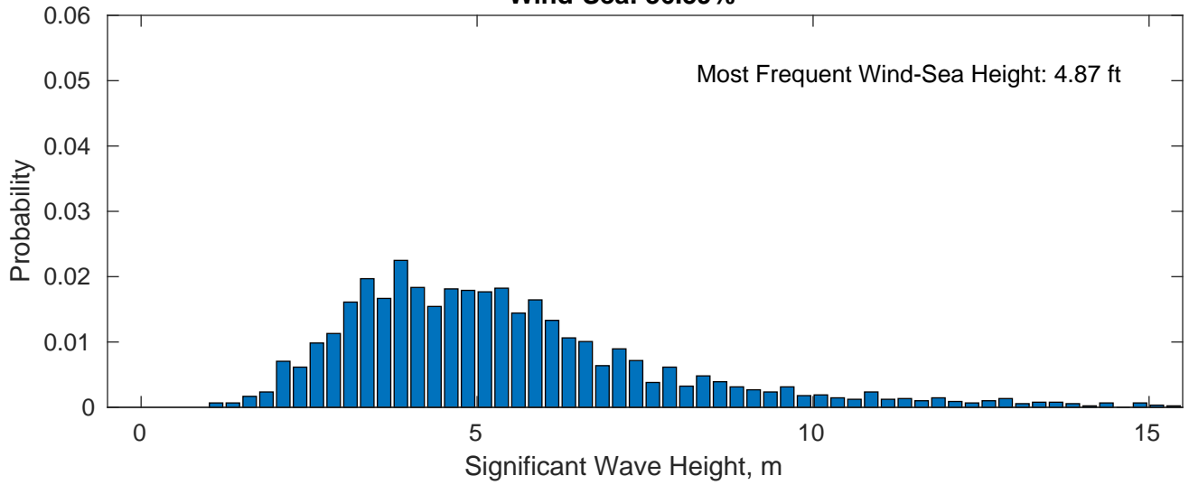
Wind-Sea: 36.59%
