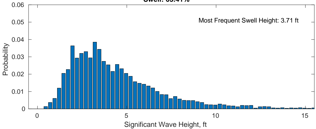
Swell: 63.41%
