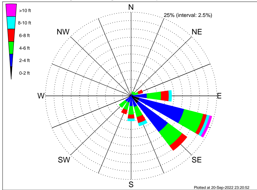
OCS-A 0537 Climatological WaveHeight Rose for September: 1979 - 2015
