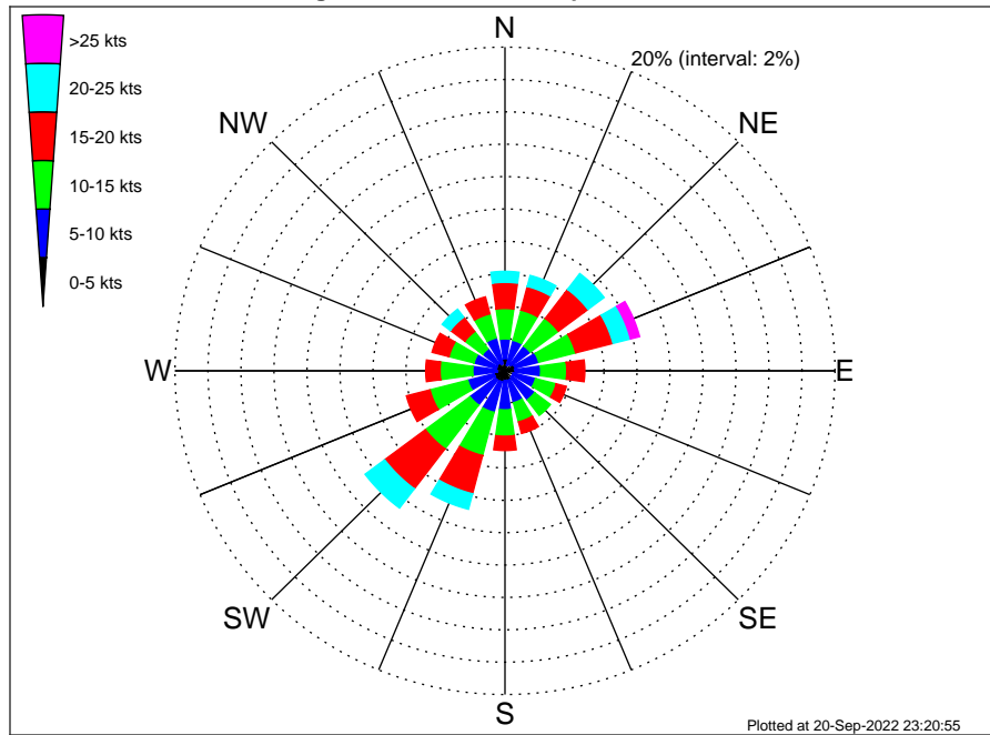
OCS-A 0537 Climatological Wind Rose for September: 1979 - 2015
