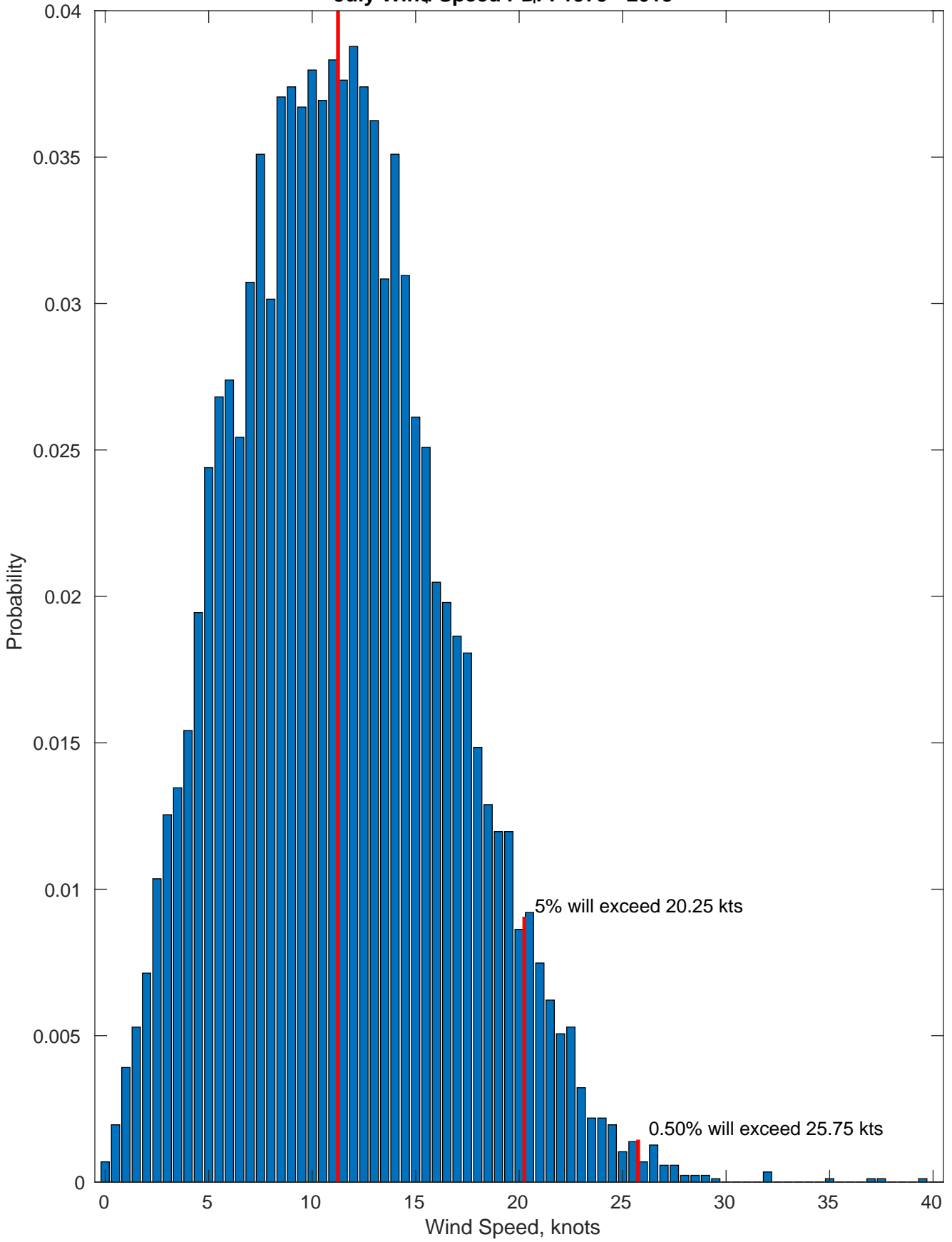
July Wind Speed PDF for 1979-2015
