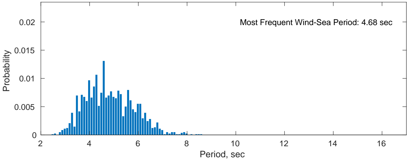
Wind-Sea: 21.77%
