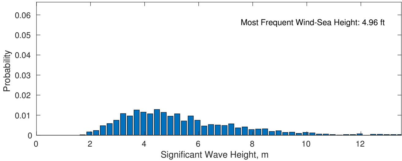
Wind-Sea: 20.93%
