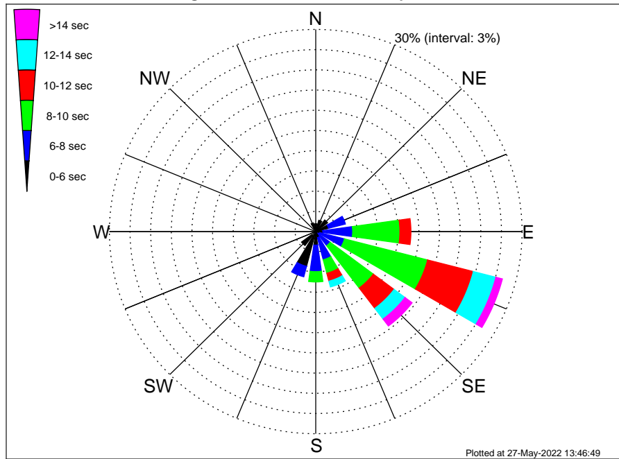
OCS-A 0538 Climatological WavePeriod Rose for September: 1979 - 2015
