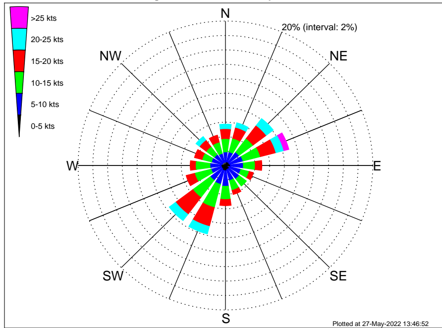
OCS-A 0538 Climatological Wind Rose for September: 1979 - 2015
