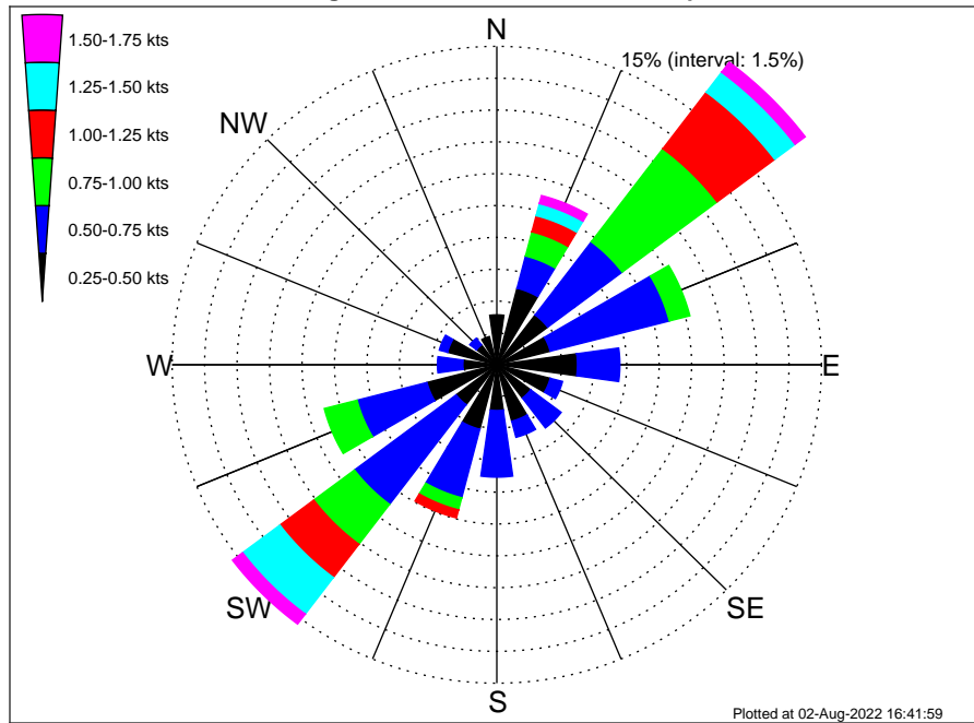
Orsted OCW02 Climatological Surface Current Rose for April: 1995 - 2012
