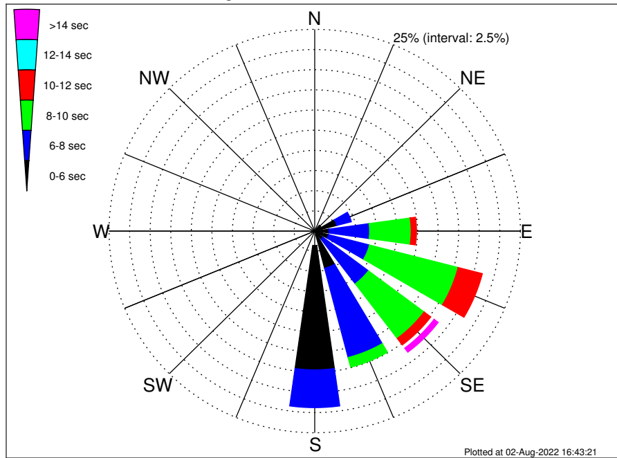
Orsted OCW02 Climatological WavePeriod Rose for June: 1979 - 2015
