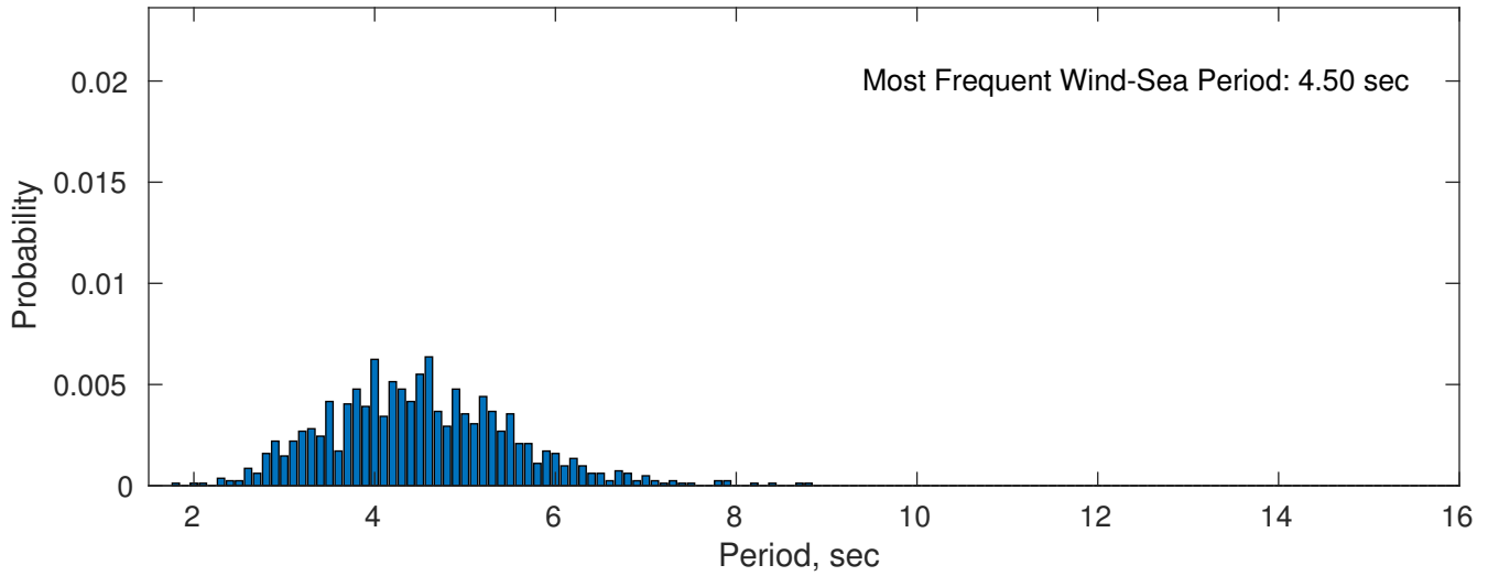
Wind-Sea: 12.19%
