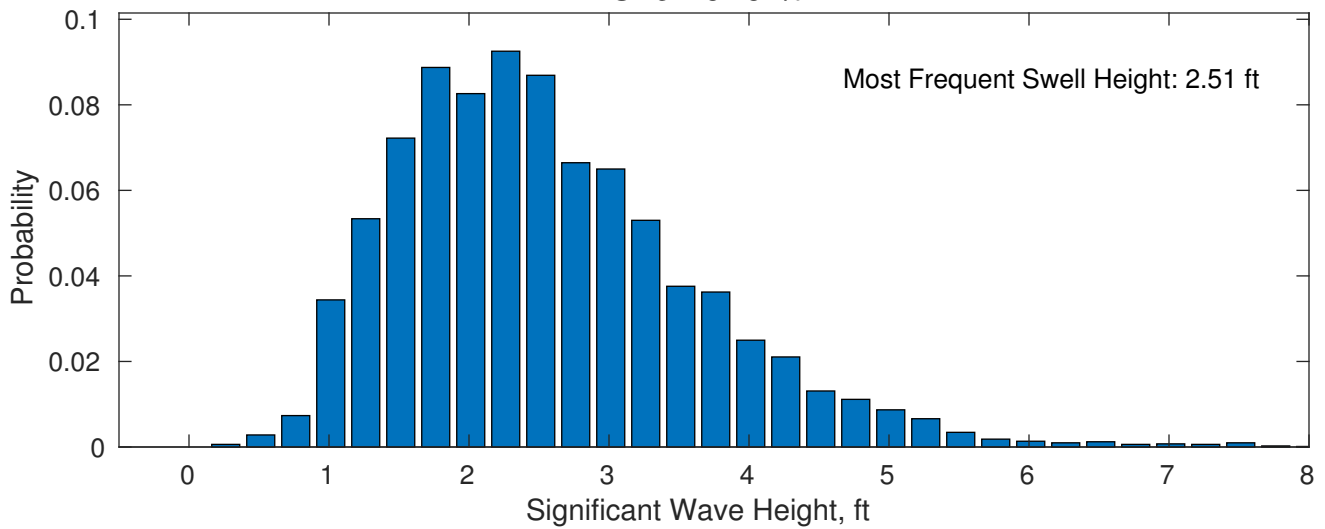
Swell: 87.81%
