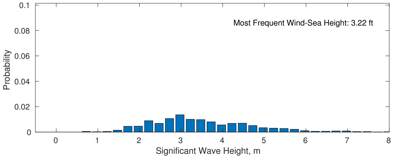
Wind-Sea: 12.19%
