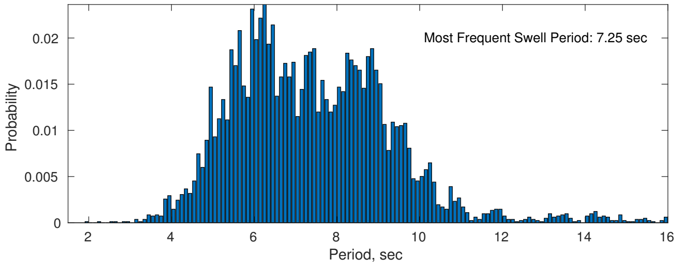
Swell: 87.81%
