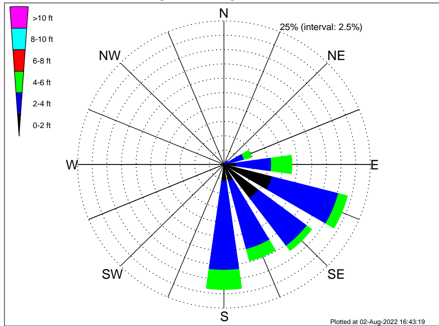
Orsted OCW02 Climatological WaveHeight Rose for June: 1979 - 2015
