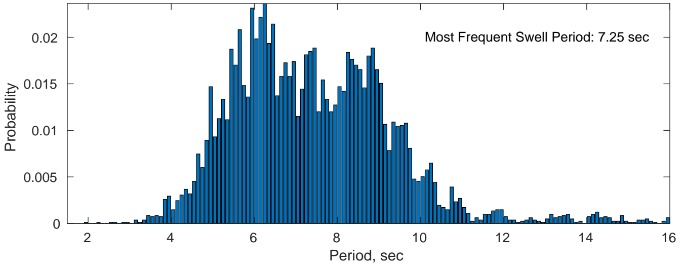
Swell: 87.81%
