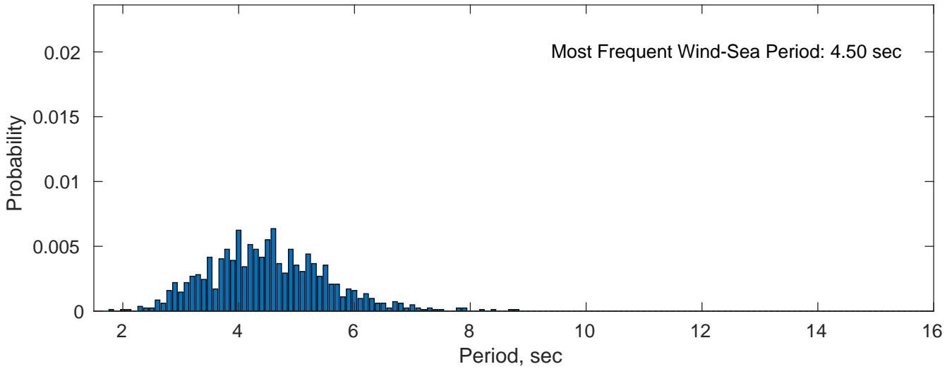
Wind-Sea: 12.19%
