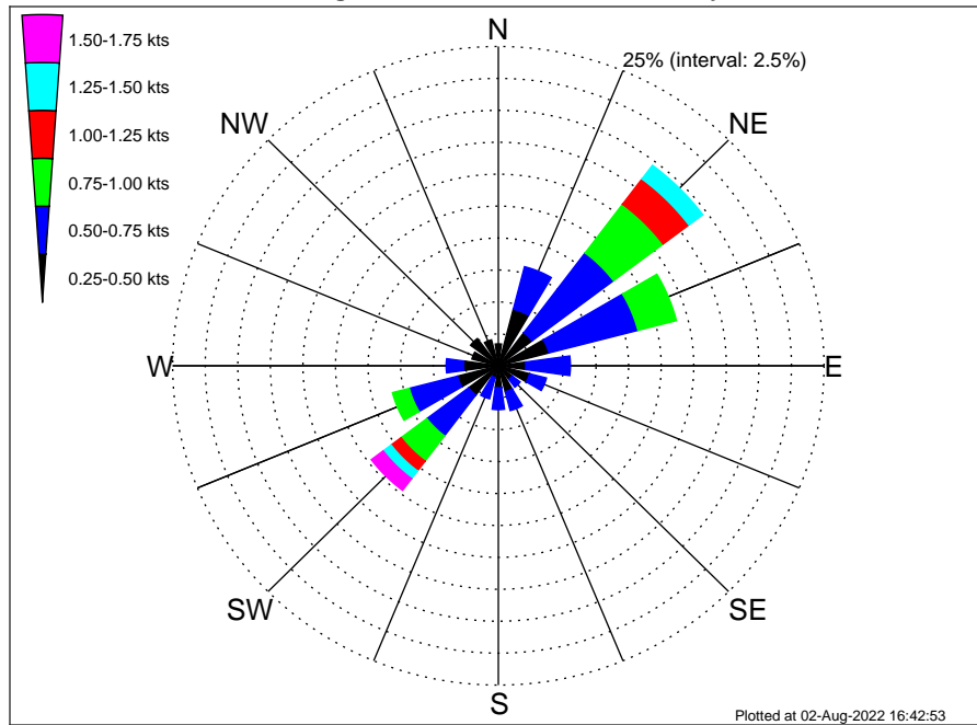
Orsted OCW02 Climatological Surface Current Rose for May: 1995 - 2012
