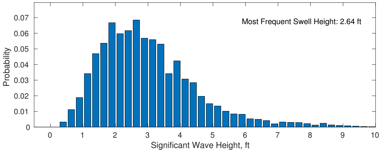
Swell: 83.73%
