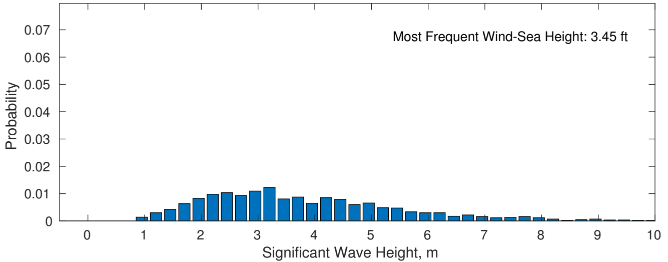
Wind-Sea: 16.27%
