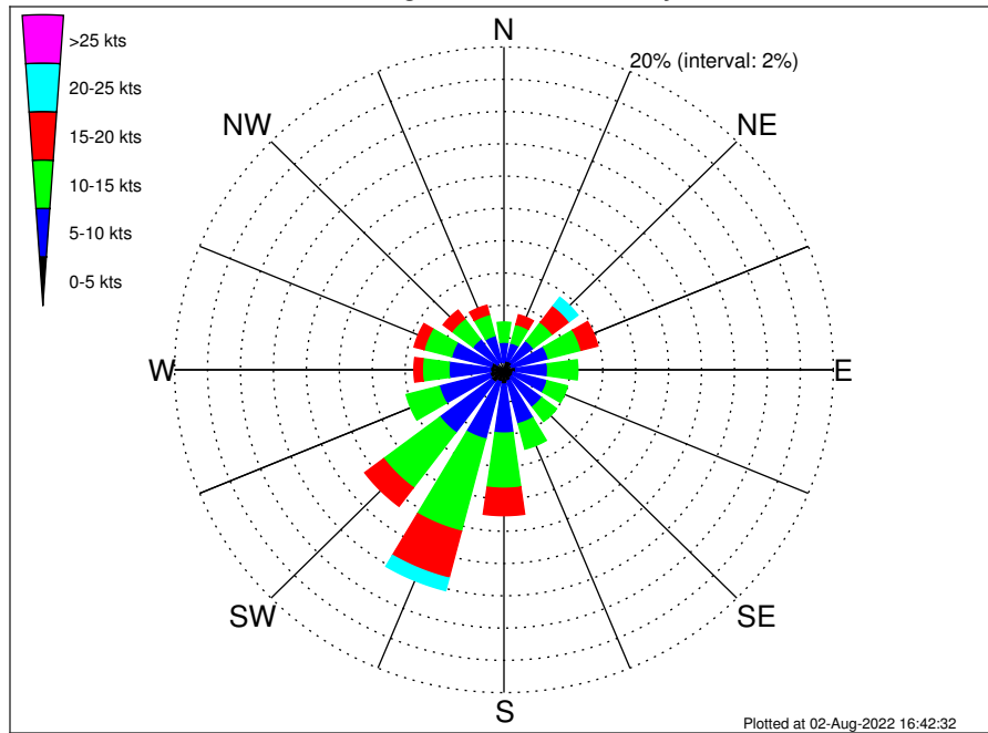
Orsted OCW02 Climatological Wind Rose for May: 1979 - 2015
