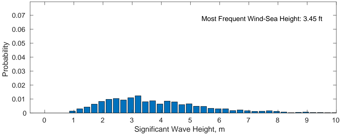
Wind-Sea: 16.27%
