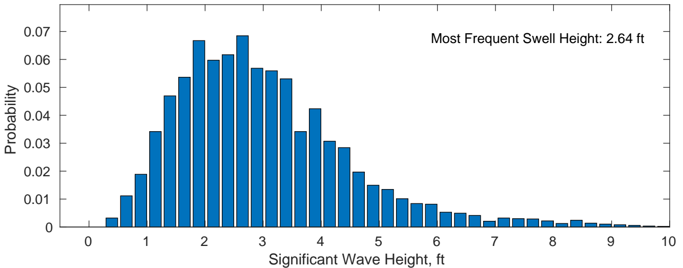
Swell: 83.73%
