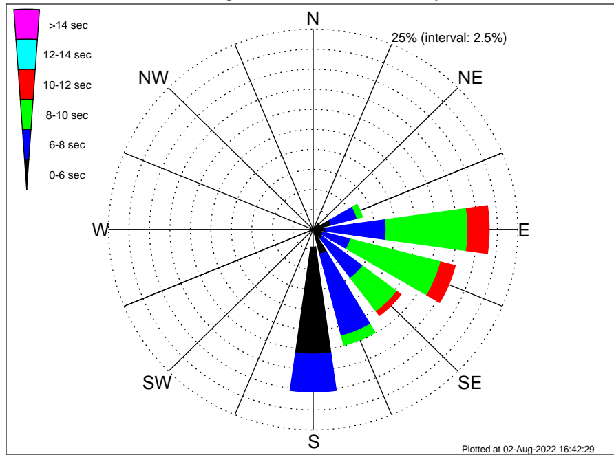
Orsted OCW02 Climatological WavePeriod Rose for May: 1979 - 2015
