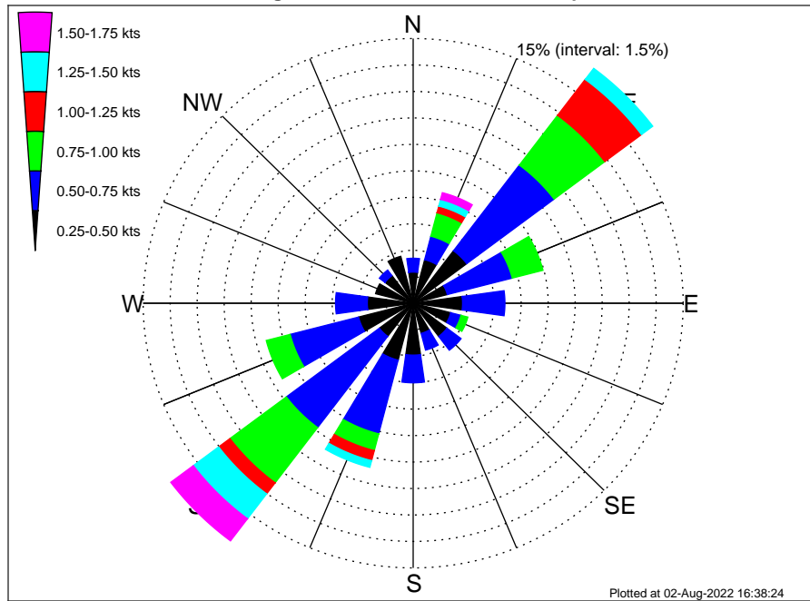
Orsted SJW02 Climatological Surface Current Rose for April: 1995 - 2012
