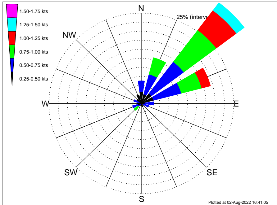
Orsted SJW02 Climatological Surface Current Rose for July: 1995 - 2012
