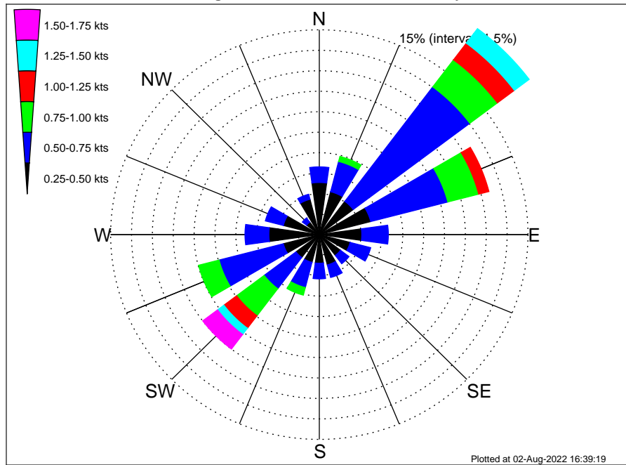
Orsted SJW02 Climatological Surface Current Rose for May: 1995 - 2012
