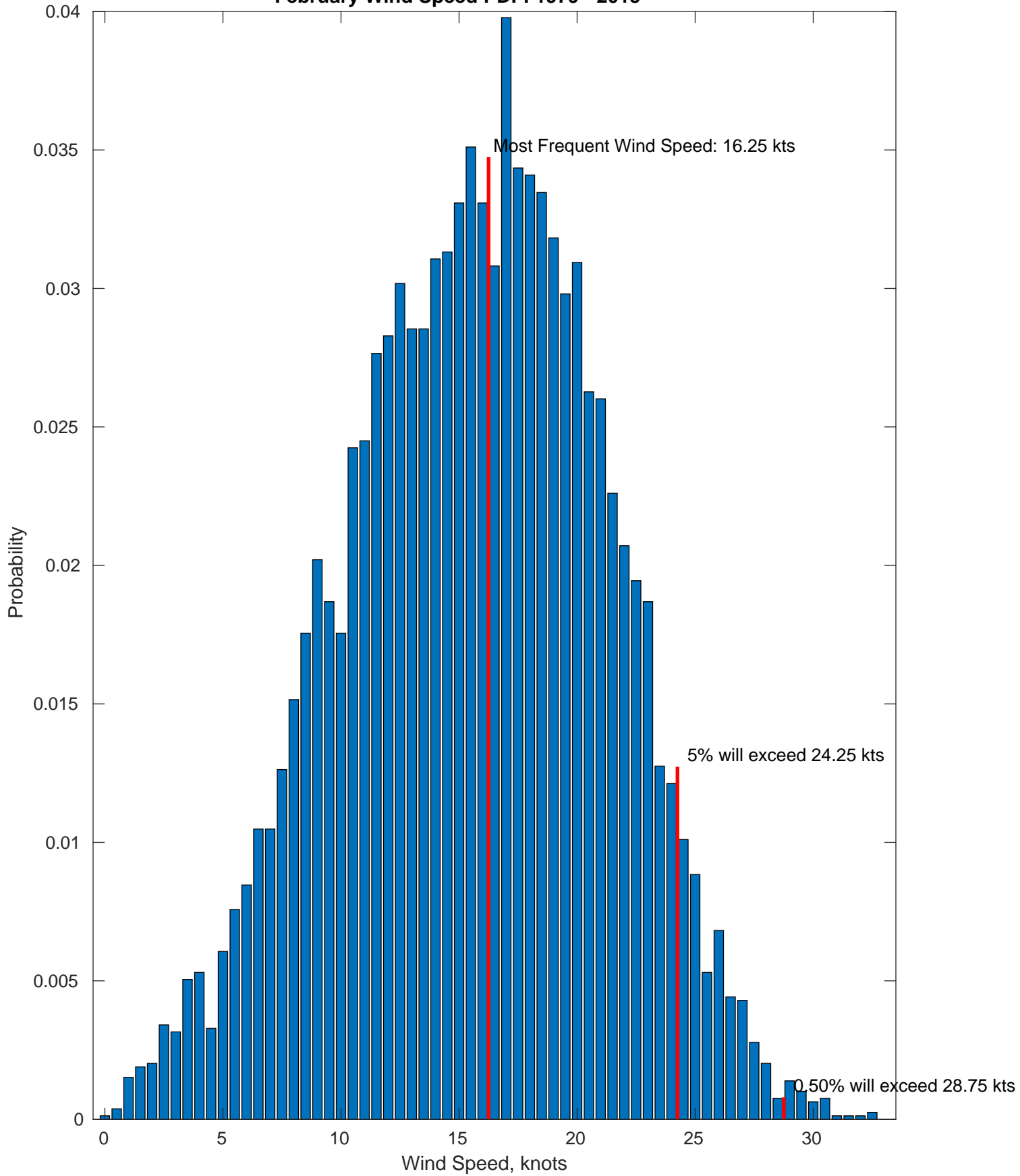
February Wind Speed PDF: 1979 - 2015
