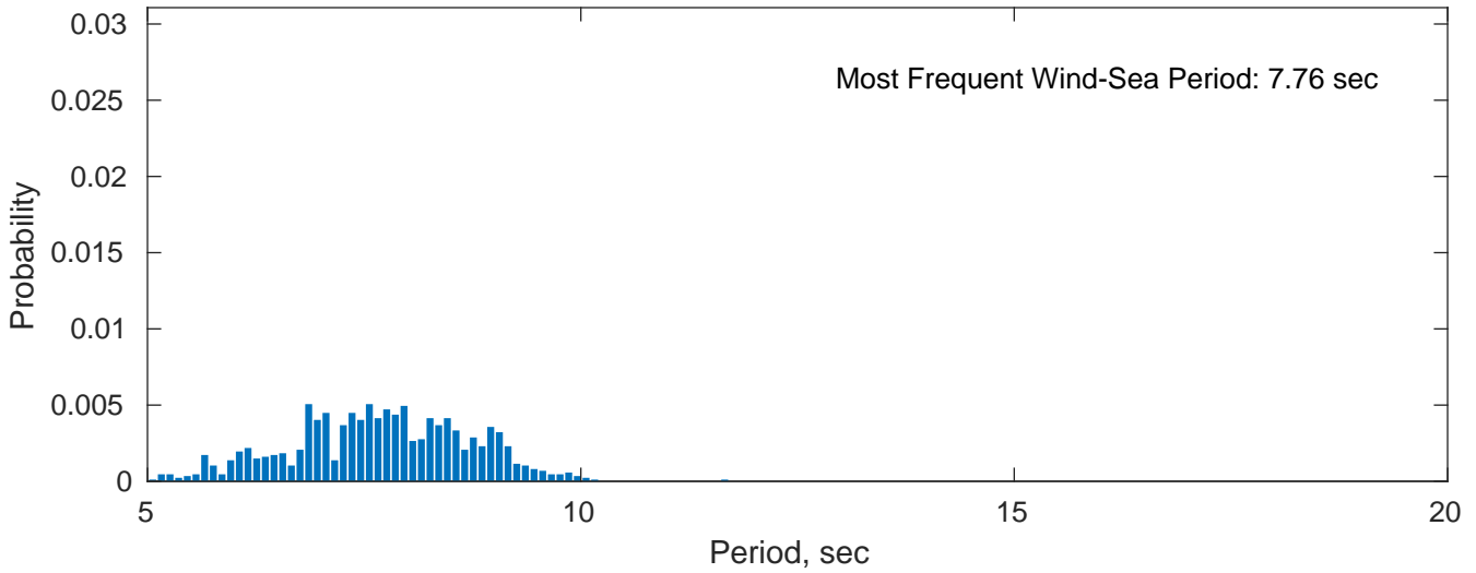
Wind-Sea: 11.41%
