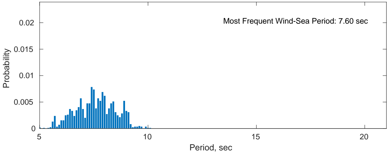
Wind-Sea: 13.64%
