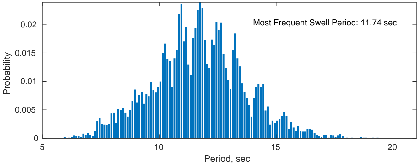
Swell: 86.36%
