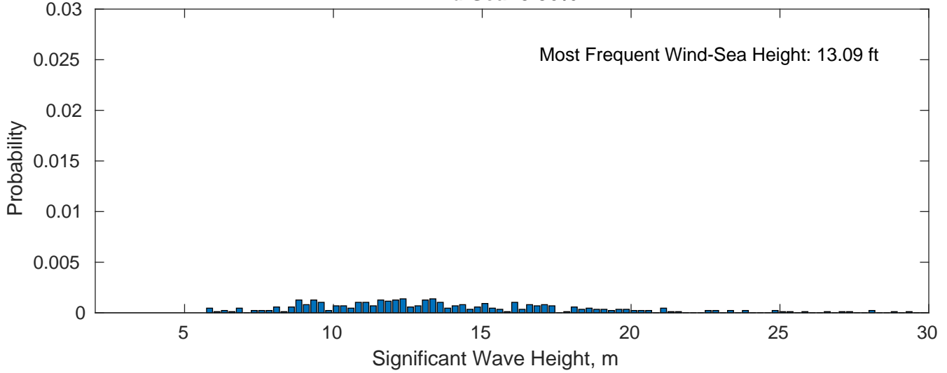
Wind-Sea: 3.86%
