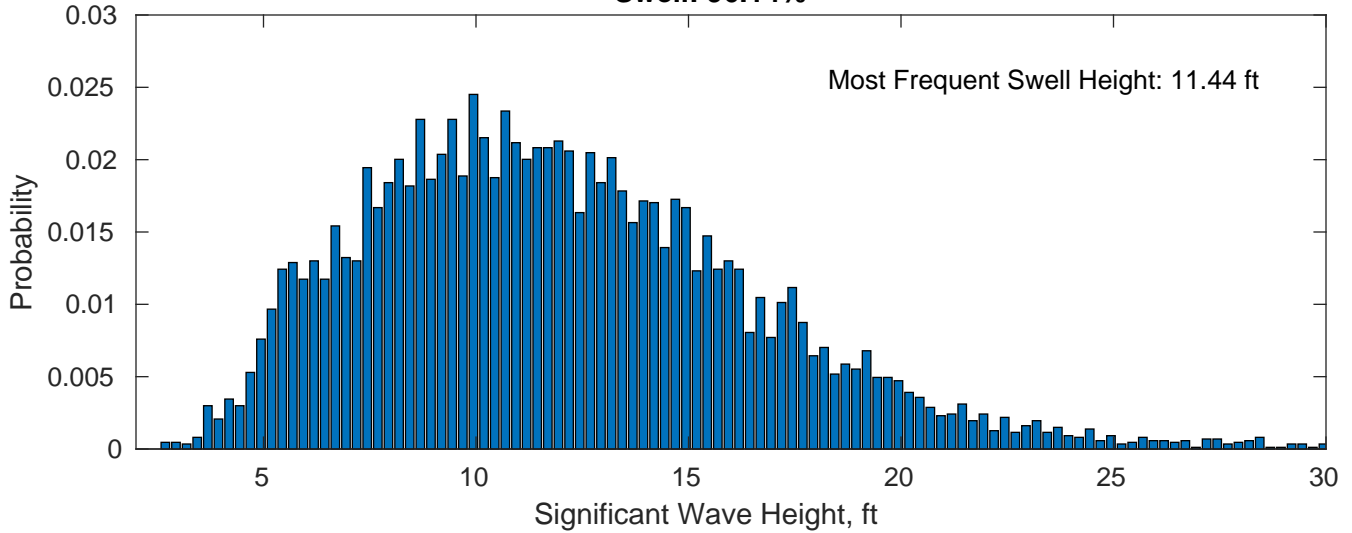
Swell: 96.14%
