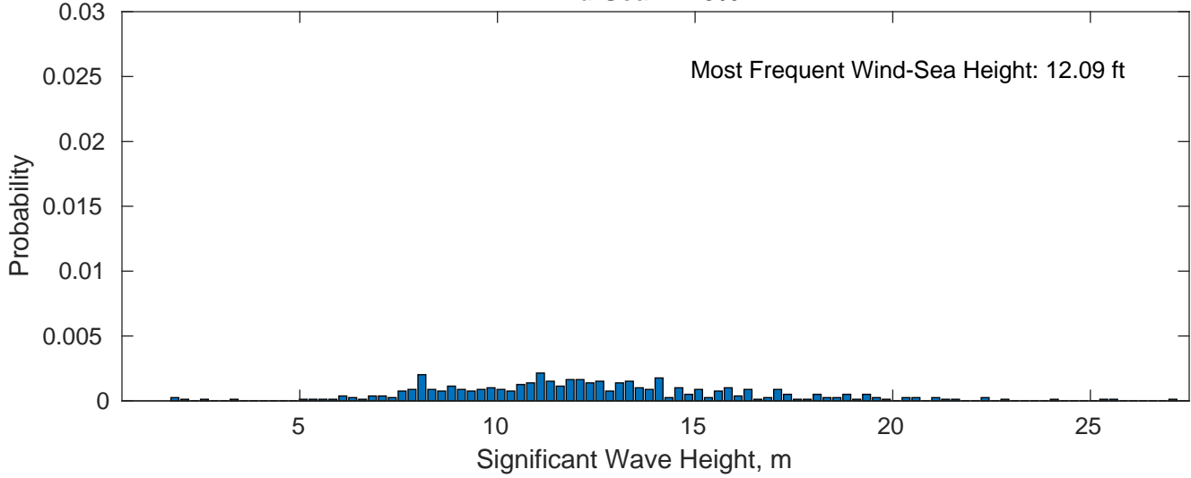
Wind-Sea: 4.78%
