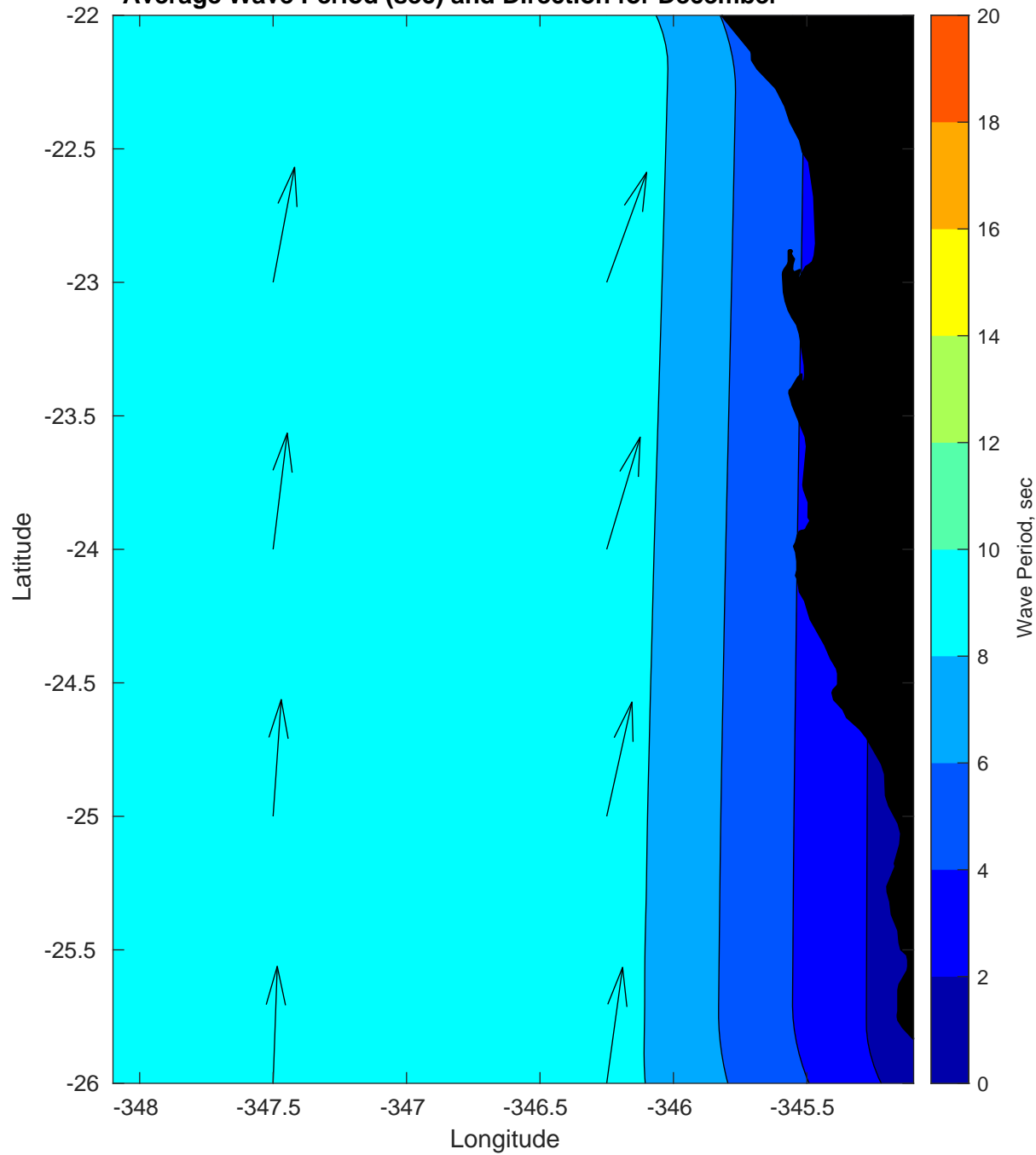
Average Wave Period (sec) and Direction for December
