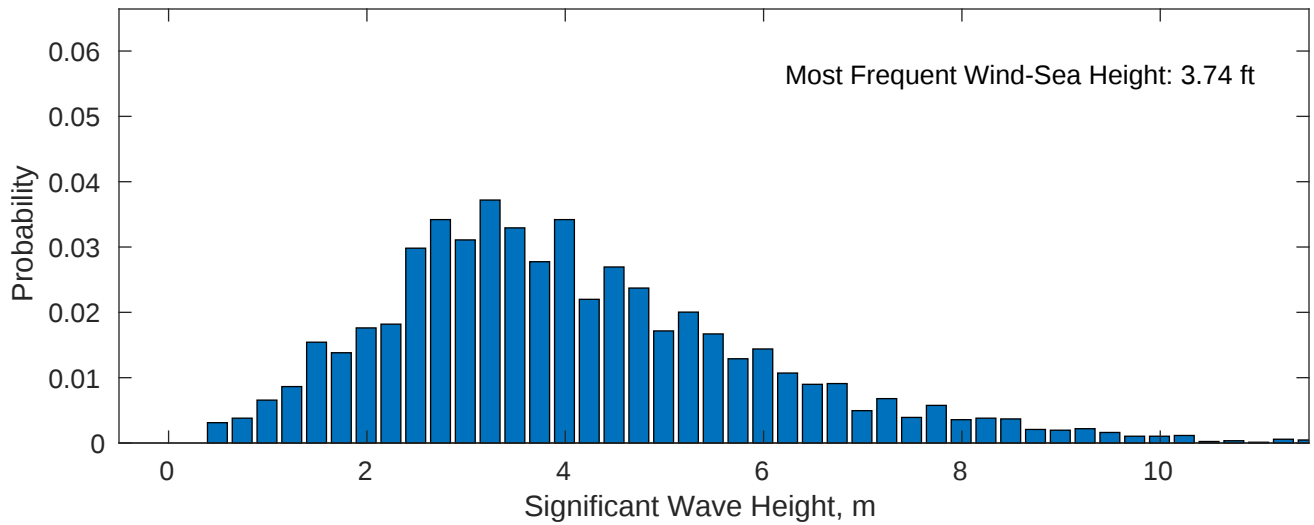
Wind-Sea: 54.23%
