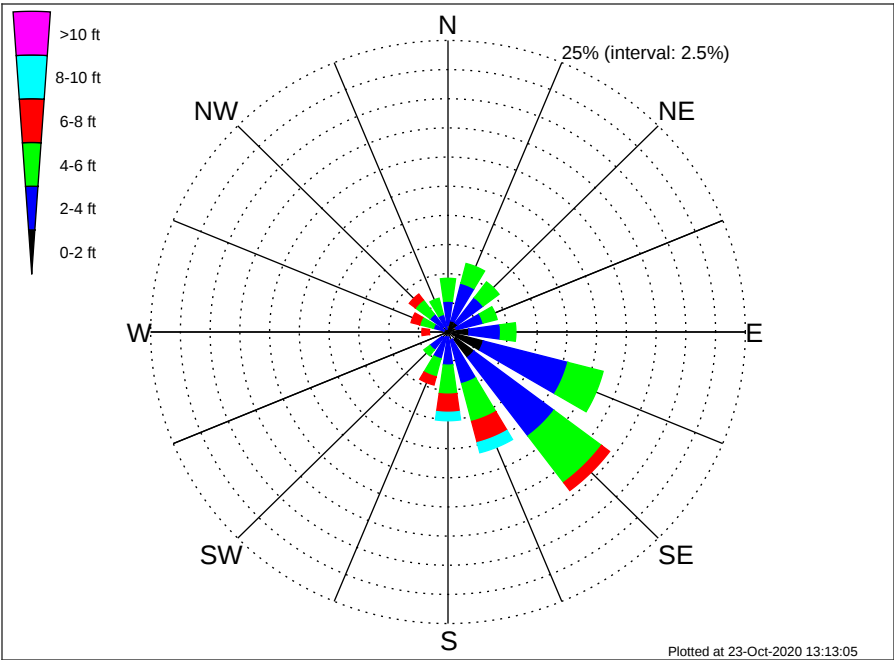
SpaceX GOM Launch Platform Climatological WaveHeight Rose for December: 1979 - 2015
