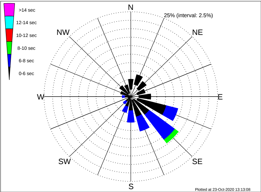
SpaceX GOM Launch Platform Climatological WavePeriod Rose for December: 1979 - 2015
